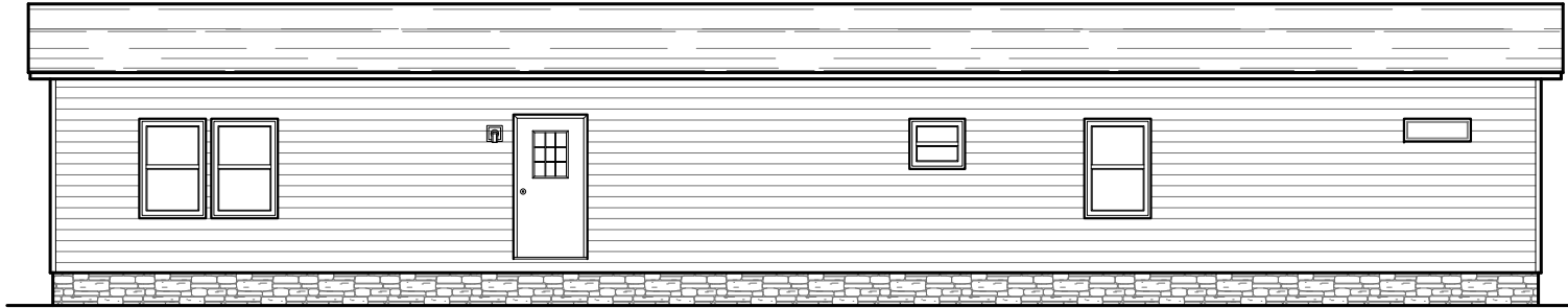
REAR ELEVATION
