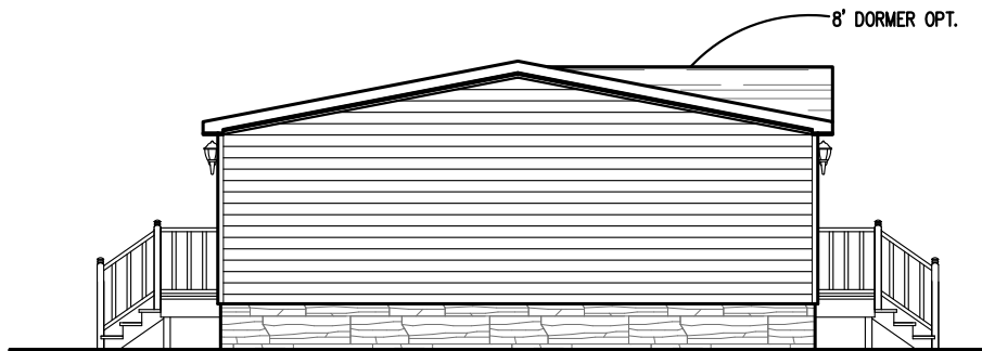
LEFT ELEVATION
