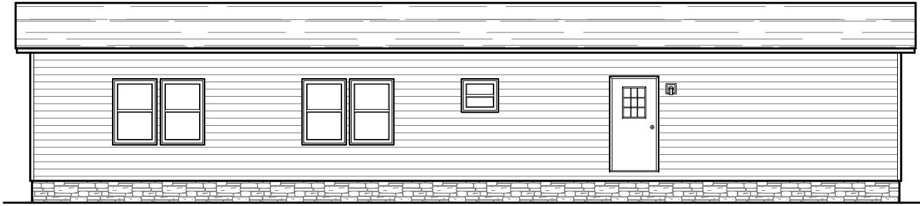
REAR ELEVATION
