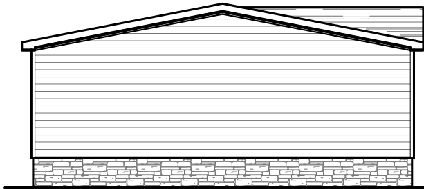
LEFT ELEVATION
